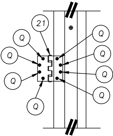
HINGE DETAIL
